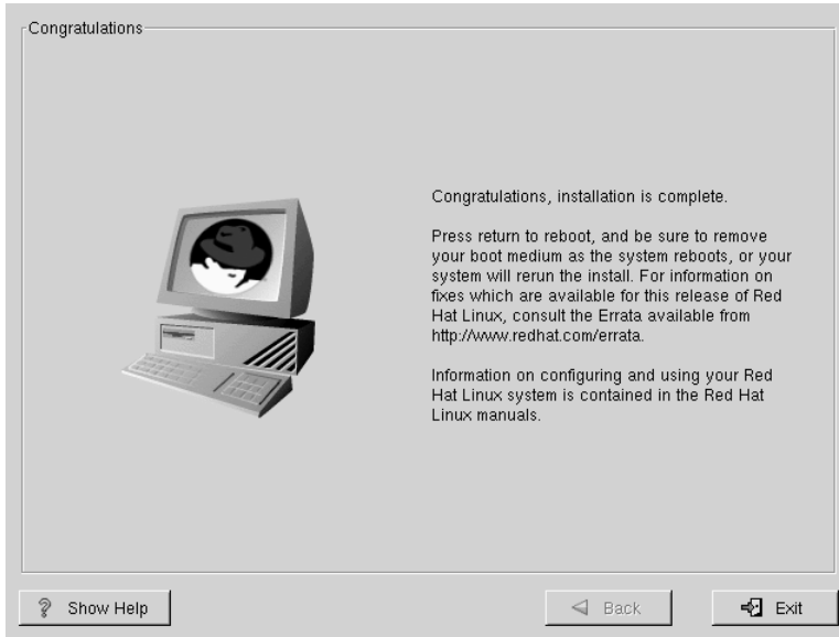
Figure 4–23 Installation Complete
