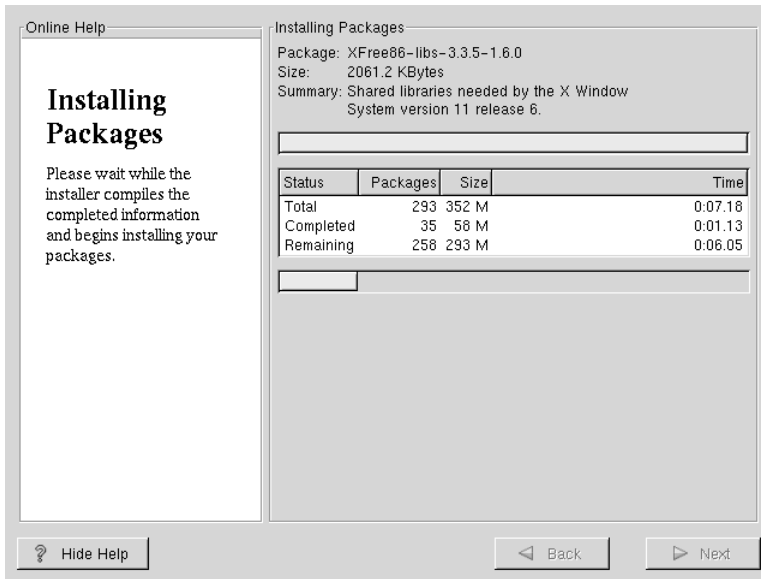
Figure 5–5 Installing Packages
