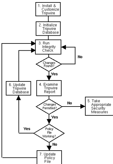
Figure 11-1. Using Tripwire
